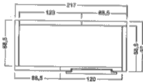
Isark 2008 Dim Int 2000 x 800 Dim Ext 2170 x 970
