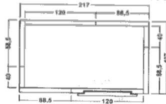
Isark 2012 Dim Int 2000 x 1200 Dim Ext 2170 x 1370
