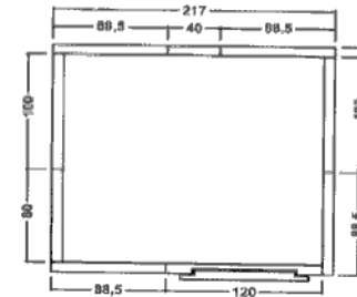
Isark 2018 Dim Int 2000 x 1800 Dim Ext 2170 x 1970
